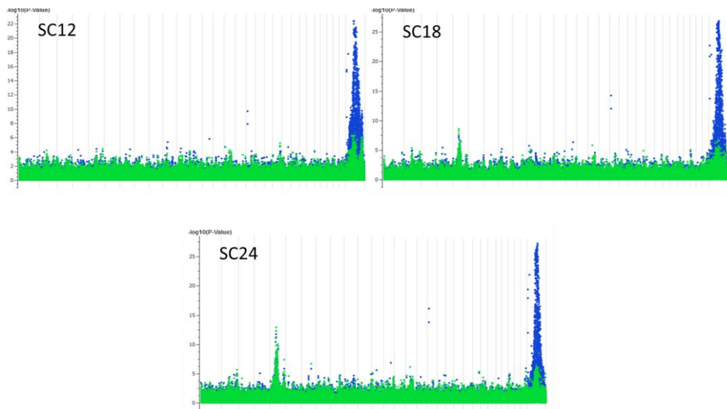
Figure 1. The association between SNP in 30 chromosome regions of beef cattle and scrotal circumference at 3 different ages. The chromosomal positions are in the x-axis and -\text{Log}(P\text{-values}) are in the y-axis. The blue indicates effect of all SNP on SC, the green reveals effect of SNP on SC with Tex11-r38k as a fixed effect.
